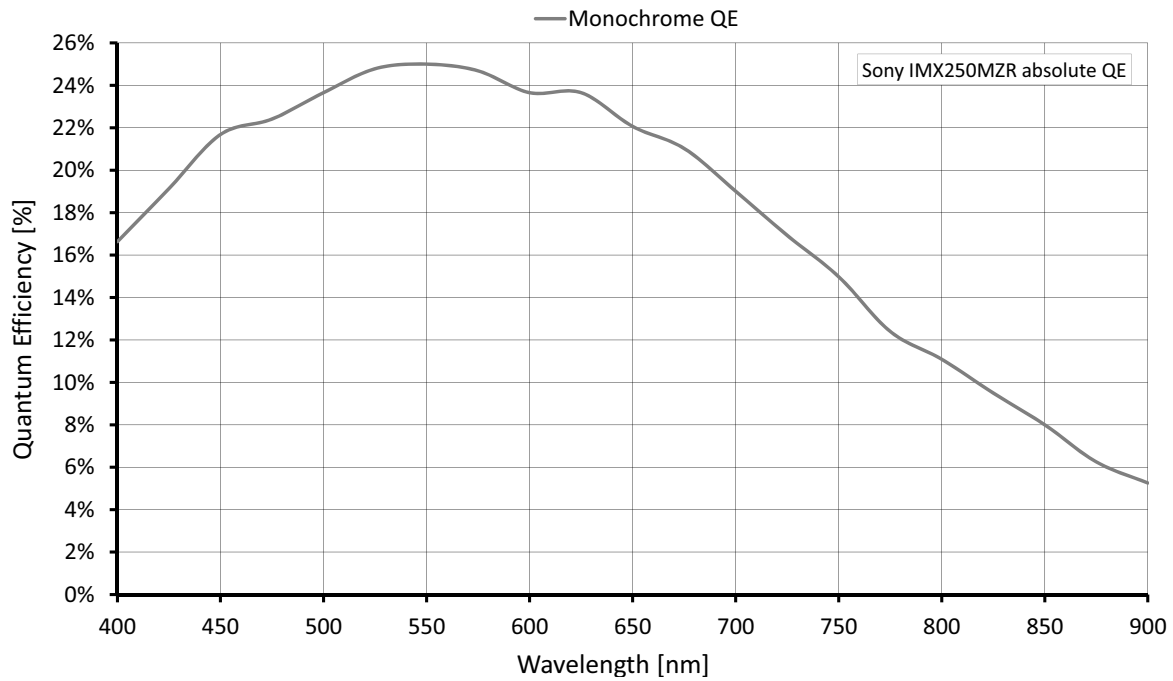
Figure 41: Mako G-508B POL (Sony IMX250MZR) absolute QE
