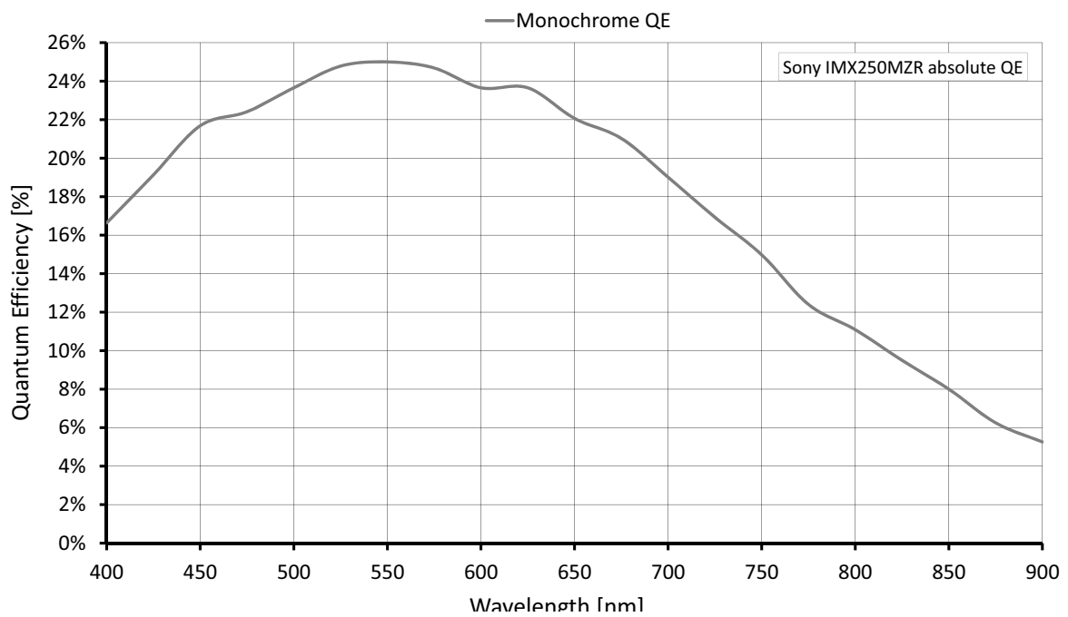
Figure 42: Mako G-508B POL (Sony IMX250MZR) spectral response
