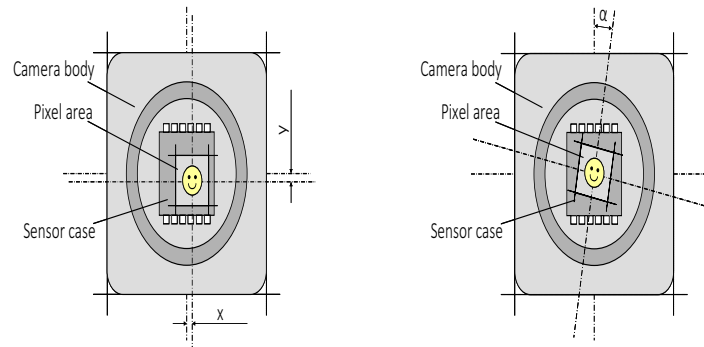
Figure 56: Sensor position accuracy
